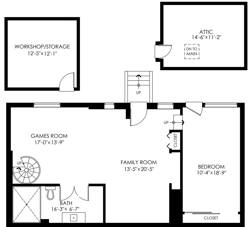
Lower Floor Plan Floor Area: 947 sq.ft. Ceiling Height: 6'-11"
